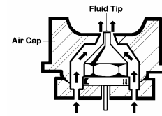
Figure 2 - Suction Feed Air Cap
