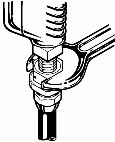
Figure 4 - Threaded-Type Connection
