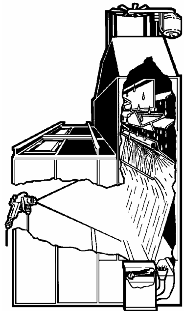
Figure 2 - Waterwash Type Spray Booth
