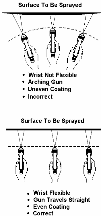
Figure 19 - Spray Techniques
