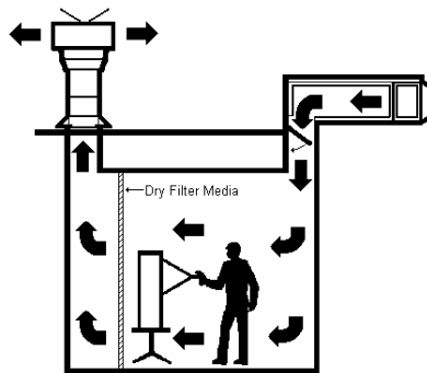
Figure 5 - Air Replacement Unit
