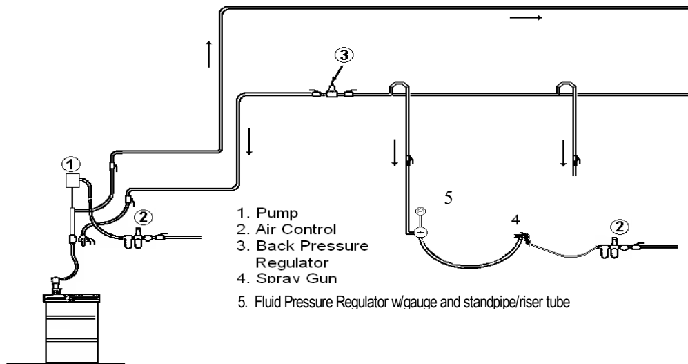
Figure 1 – Circulating System
